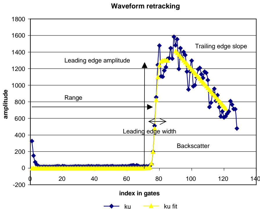
Fig. 1. The altimetric waveform is represented in blue and the fitting function from the retracking in yellow. The different parameters extracted from the altimetric waveform are described.
